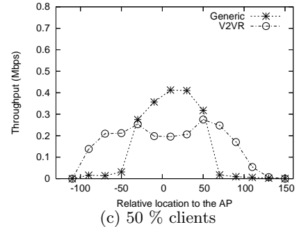
Figure 13: Vehicle TCP data transmission throughput at different distances.
