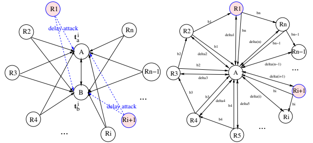
Fig. 2. Two models for secure time synchronization
